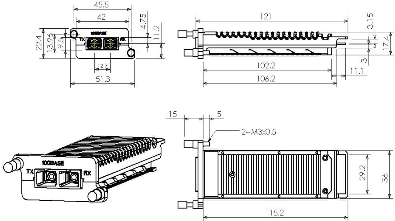
Figure 1 Mechanical dimensions
